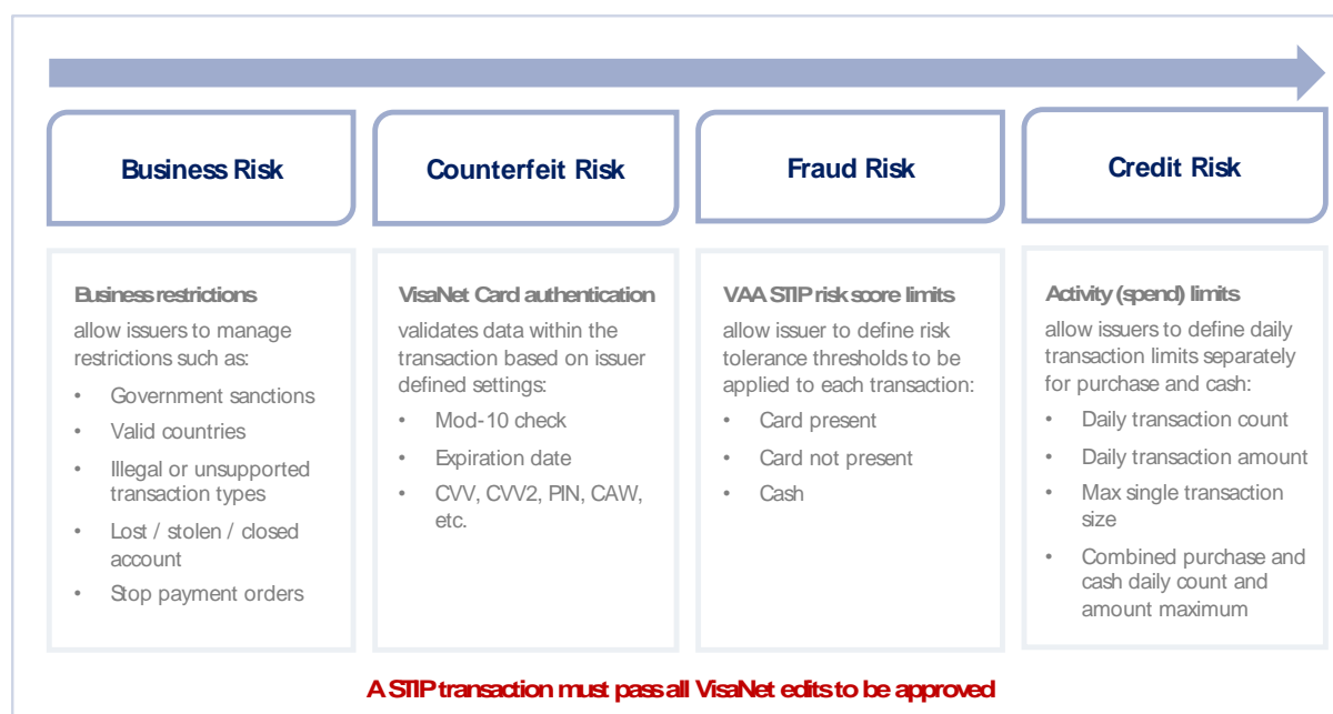
Figure 18: The VisaNet STIP service offers a robust set of parameters to effectively manage STIP risk, including:
