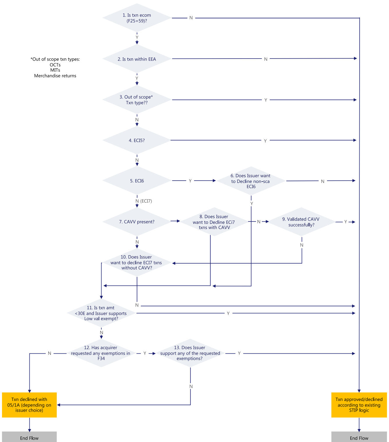
Figure 20: STIP SCA flowchart
