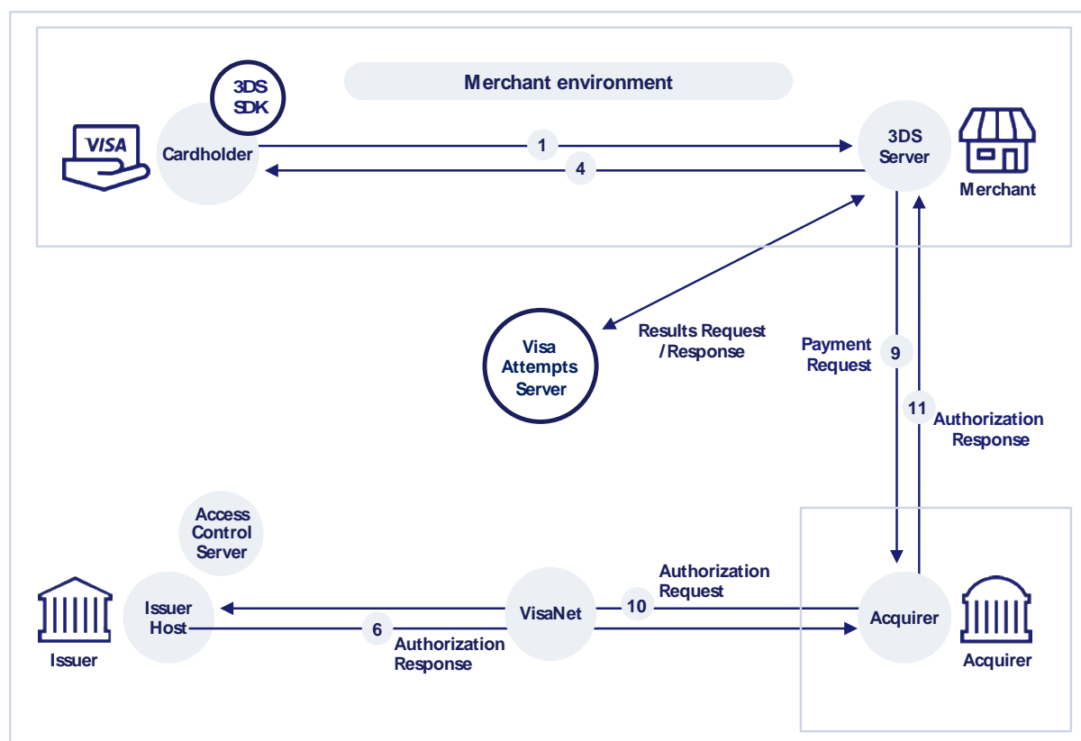
Figure 16: The role of the Visa Attempts Server
